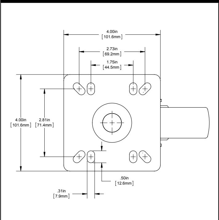
CMPU SERIES MOUNTING PLATE
