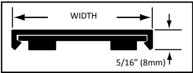
MODEL NO. T55-20-011 2-5/16" (59mm) WIDE
