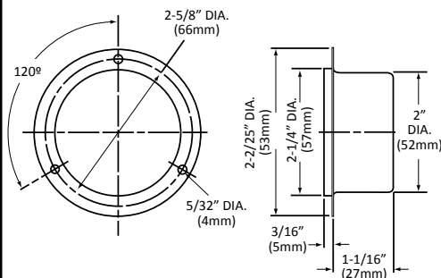
FLUSH FRONT RECESSED MOUNT THERMOMETER MODEL NO. T90-6142
