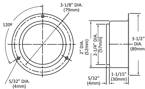
SURFACE MOUNT THERMOMETER MODEL NO. T90-6812
