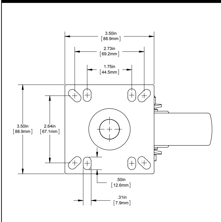
CMP4 SERIES MOUNTING PLATE
