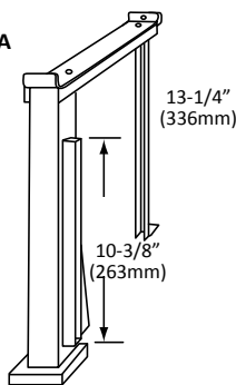
MODEL NO. J25-2100 (LEFT HAND)
