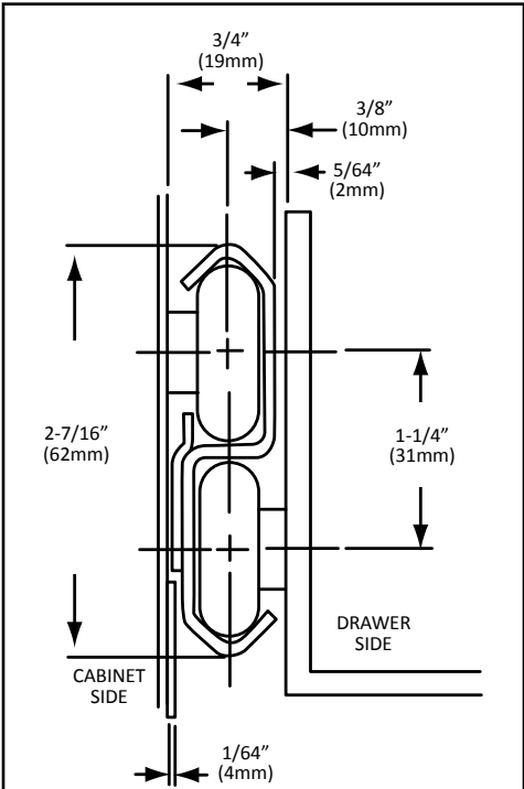
CROSS SECTION WHEN ORDERING...MEASURE FROM INSIDE FACE TO EXTREME REAR OF DRAWER
