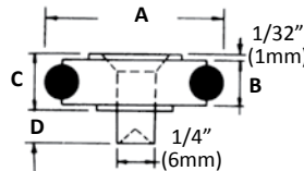
RUBBER TIRE BEARING WITH RIVET STUD STEEL INNER AND OUTER RACE
