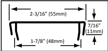
MODEL NO. T55-20-010 2-3/16" (55mm) WIDE FURNISHED IN 6 ft (1830mm) LENGTHS
