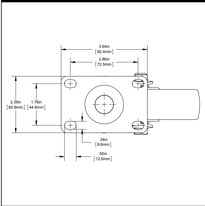
CMP1 SERIES MOUNTING PLATE
