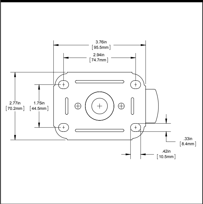
CLP2 SERIES MOUNTING PLATE
